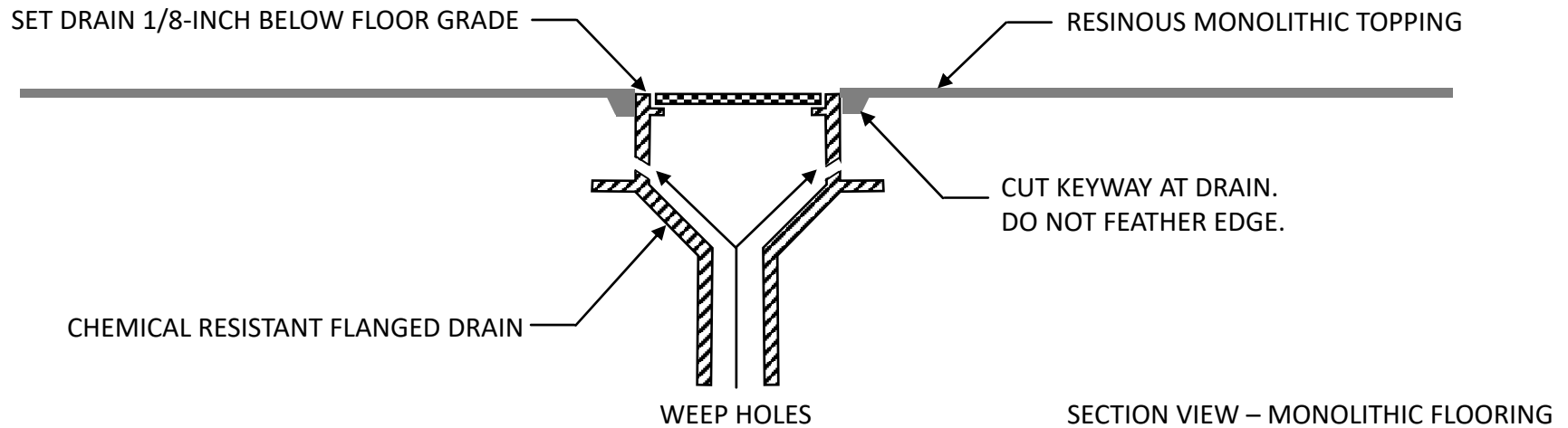
SECTION VIEW – ACID PROOF BRICK FLOORING
