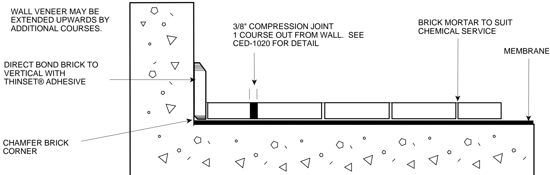
SECTION VIEW ABOVE TYPIFIES BRICK/MEMBRANE CONST'N SECTION VIEW BELOW TYPIFIES DIRECT BOND CONST'N
