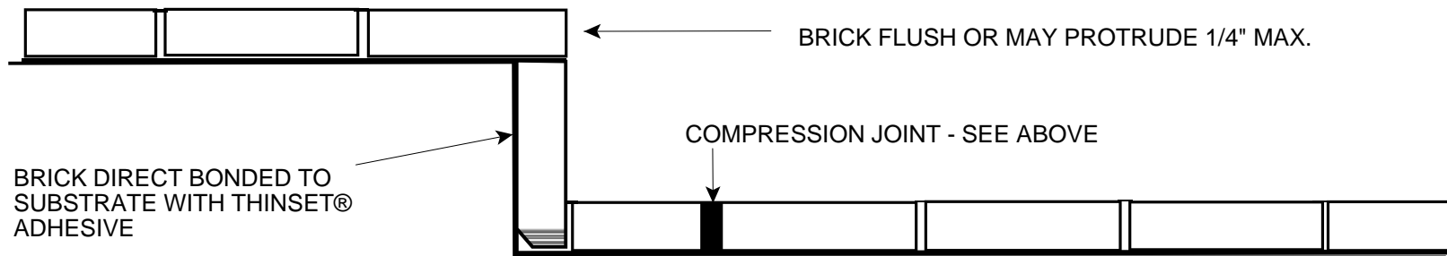
SECTION VIEW ABOVE TYPIFIES BRICK/MEMBRANE CONST'N SECTION VIEW BELOW TYPIFIES DIRECT BOND CONST'N
